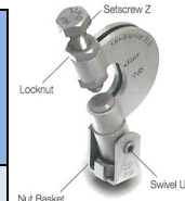
LDLFLS037: Type FLS beam flange: Beam flange clamp with swivel unit. For parallel and sloping flanges. Supplied with grade 8.8 setscrew for secure grip
